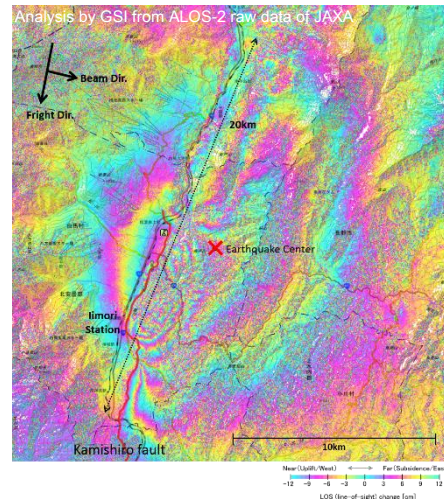
Crustal movement from the 2014 northern Nagano Prefecture earthquake captured by Interferometric SAR
